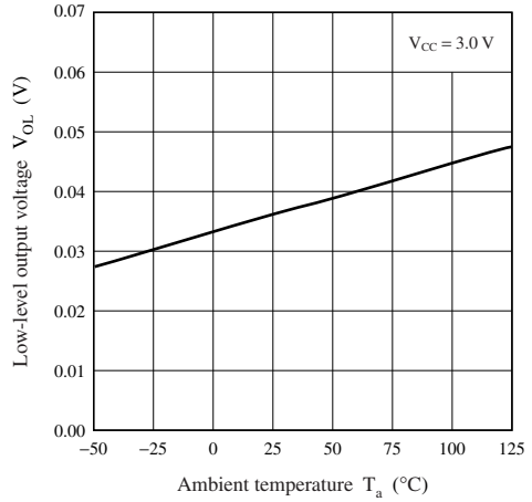
Low-level output voltage — Ambient temperature
