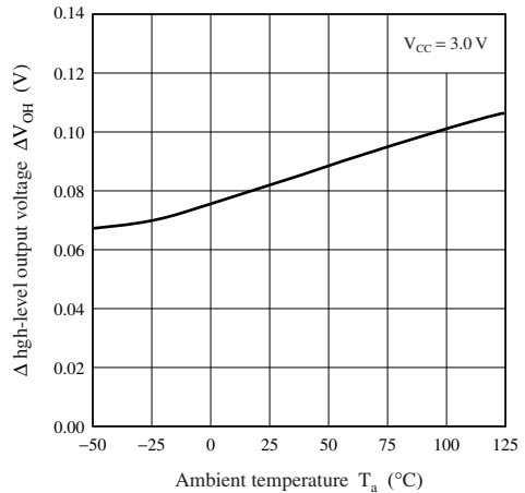
\Delta high-level output voltage — Ambient temperature
