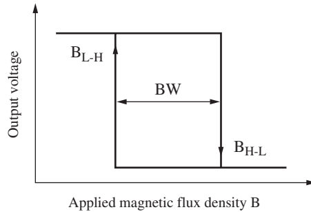
Operating magnetic flux density
