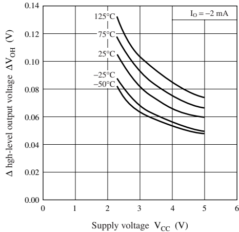
\Delta high-level output voltage — Supply voltage
